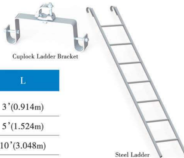
Steel Ladder
